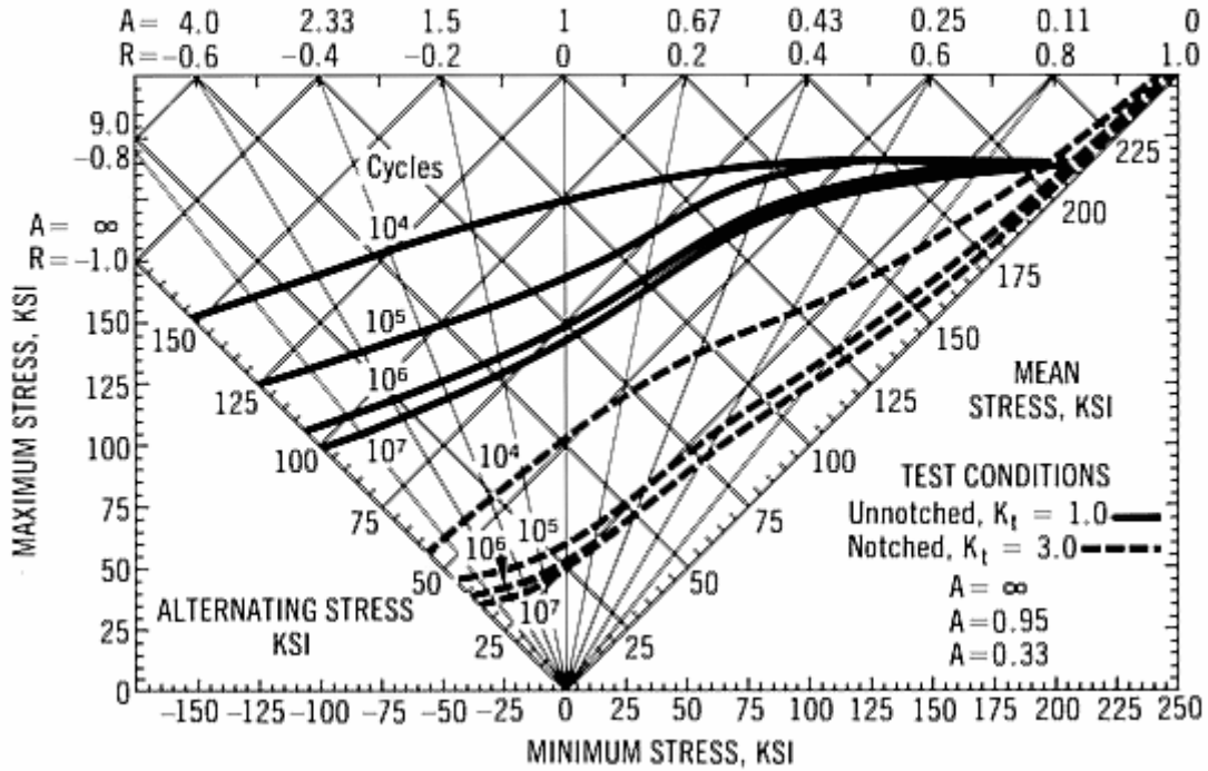
Typical Constant Life Fatigue Diagram for Custom 455 Stainless Bar in the H 1000 Condition at Room Temperature (Axial tests using longitudinal specimens)
