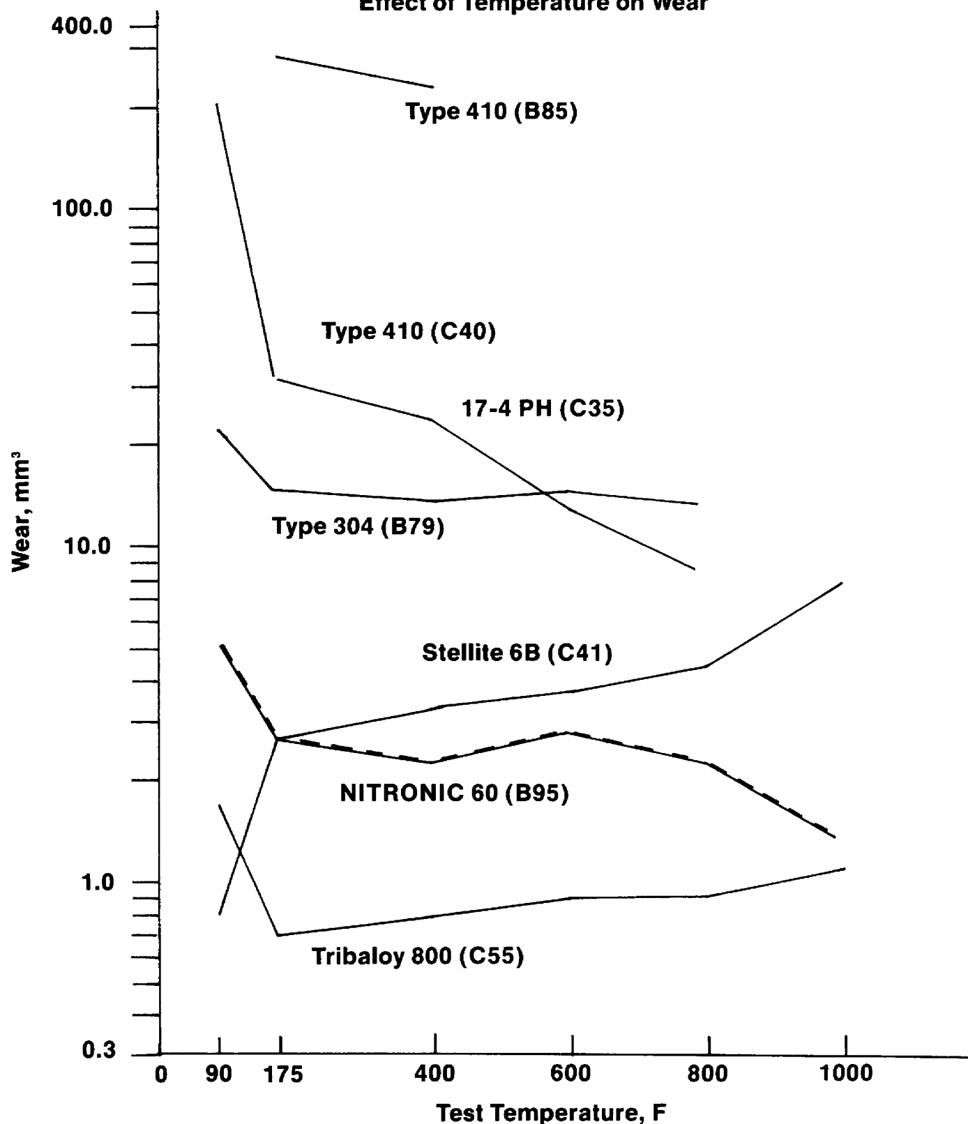
FIGURE 6 Effect of Temperature on Wear
