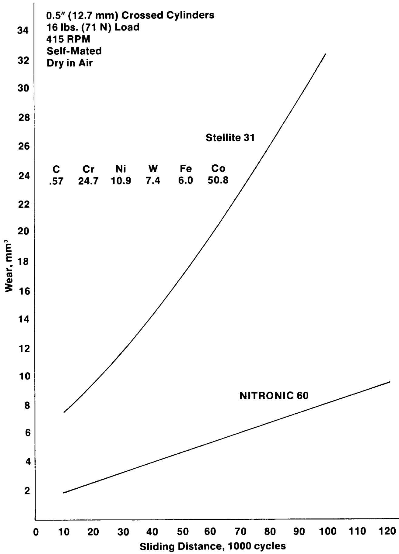
FIGURE 5 Wear of NITRONIC 60 and Stellite 31
