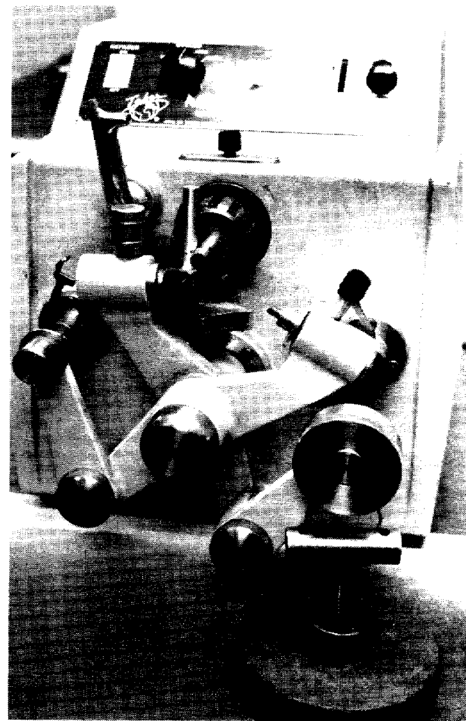
Taber Met-Abrader crossed cylinder wear test.
